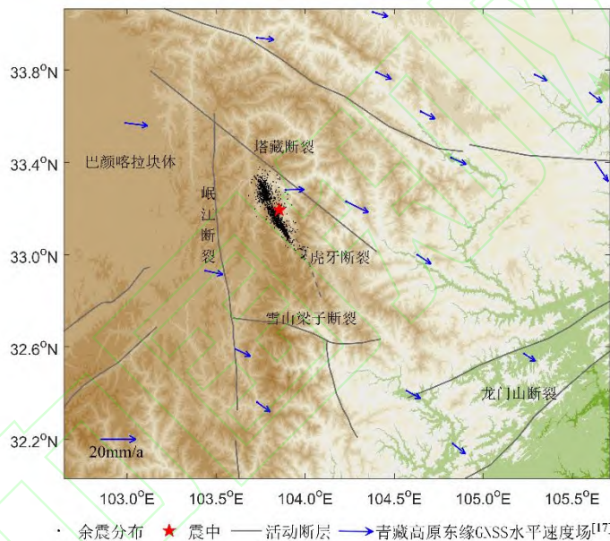
图 1 2017 年九寨沟地震构造背景图 Fig.1 Tectonic Setting of The 2017 Jiuzhaigou Earthquake.
