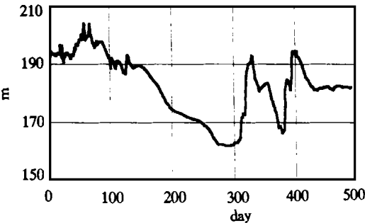
图 3 大坝上游水位波形图 Fig. 3 Water Level Wave of Geheyan Reservoir
